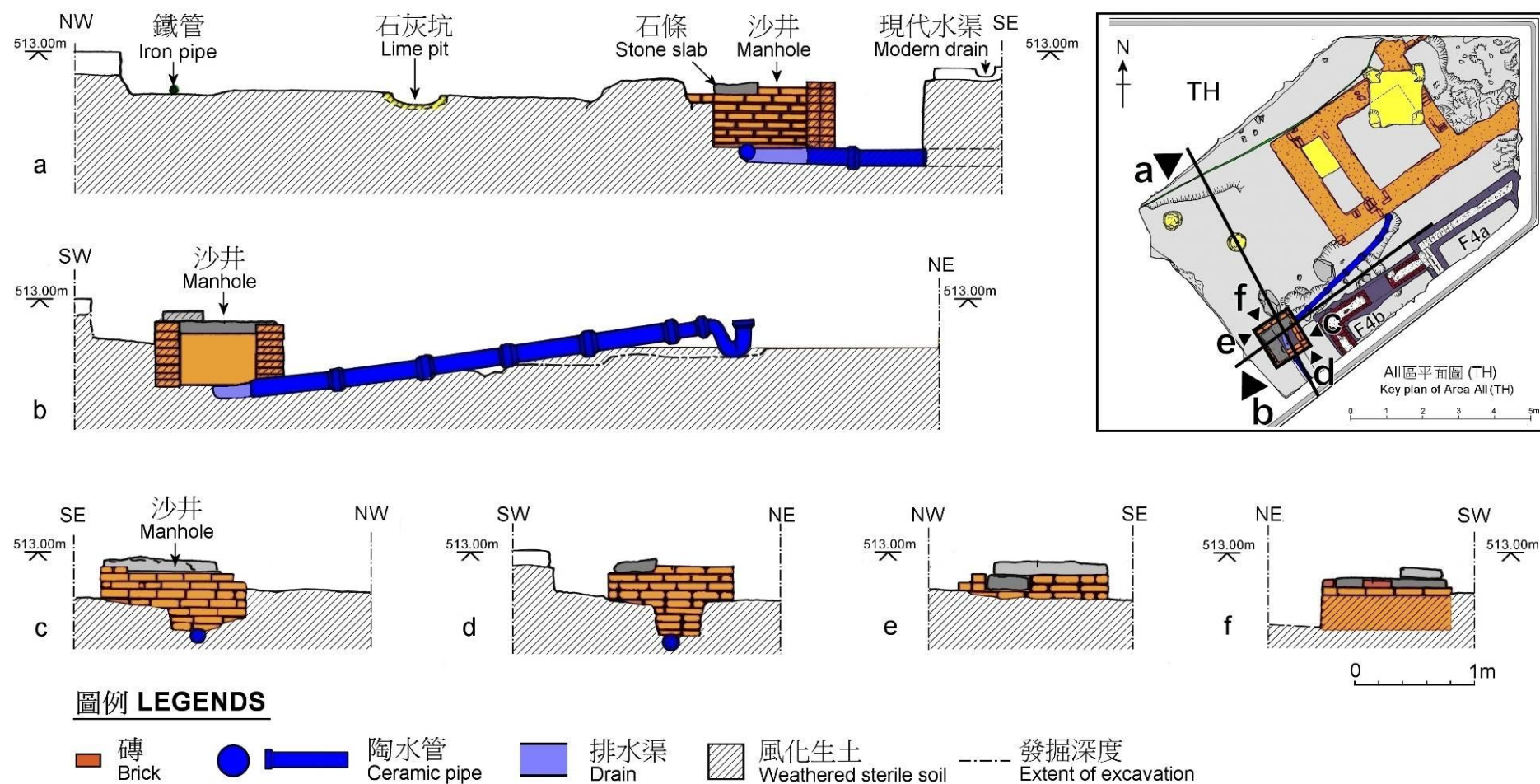
圖 18 陶水管及沙井側視剖面圖 Fig 18 Profiles & side views of ceramic pipe and manhole
