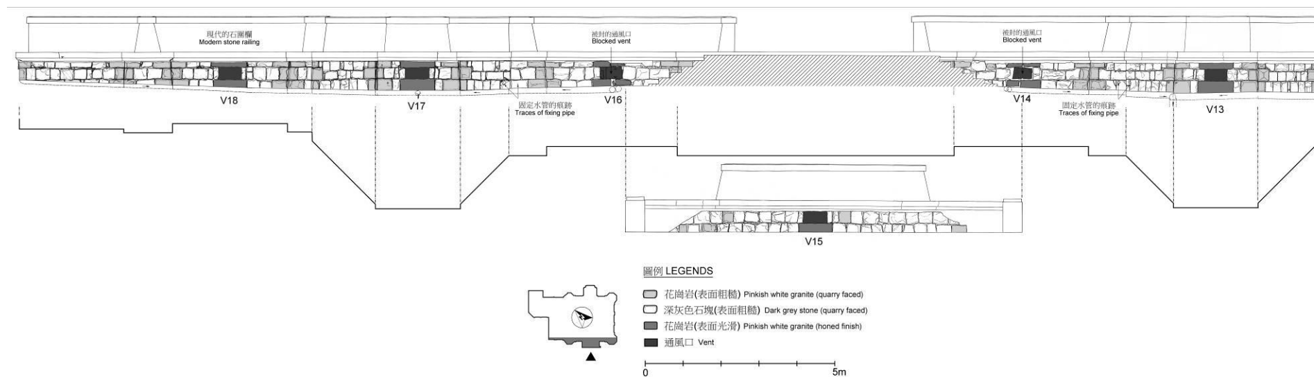
圖 30 前總督山頂別墅南面的外石牆基 Fig 30 Southern stone wall foundation of Former Mountain Lodge
