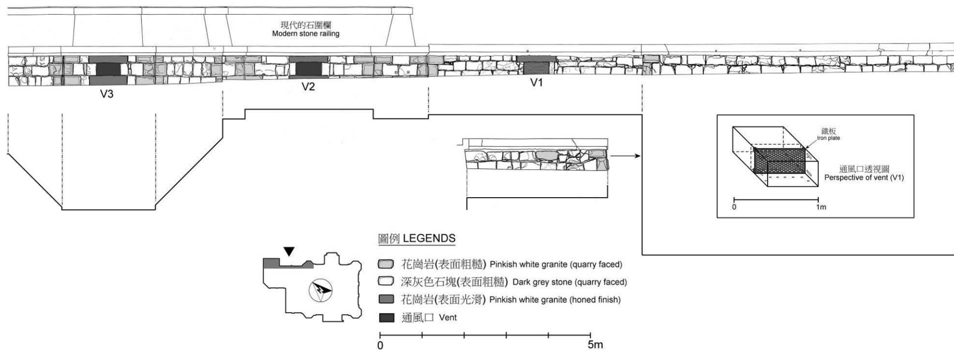
圖 27 前總督山頂別墅北面的外石牆基 (西部) Fig 27 Northern stone wall foundation of Former Mountain Lodge (western part)
