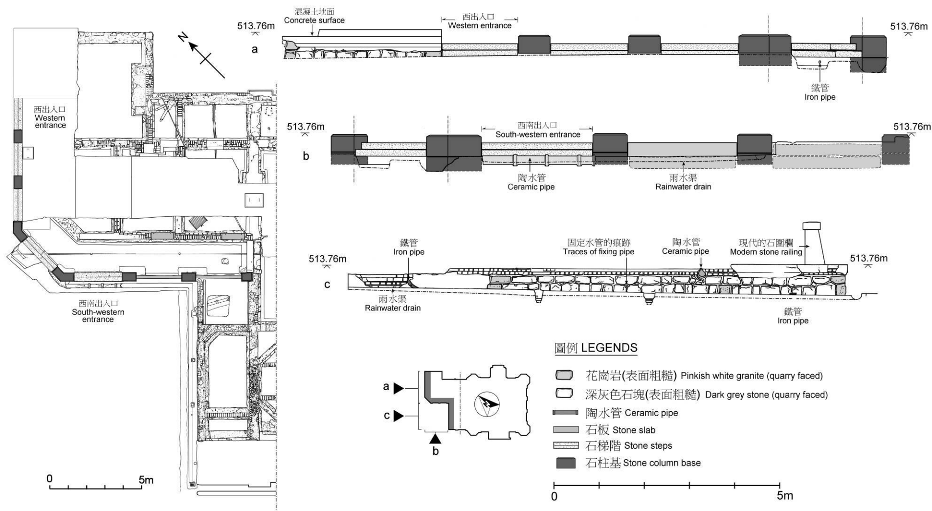
圖 31 前總督山頂別墅西面的外石牆基 Fig 31 Western stone wall foundation of Former Mountain Lodge
