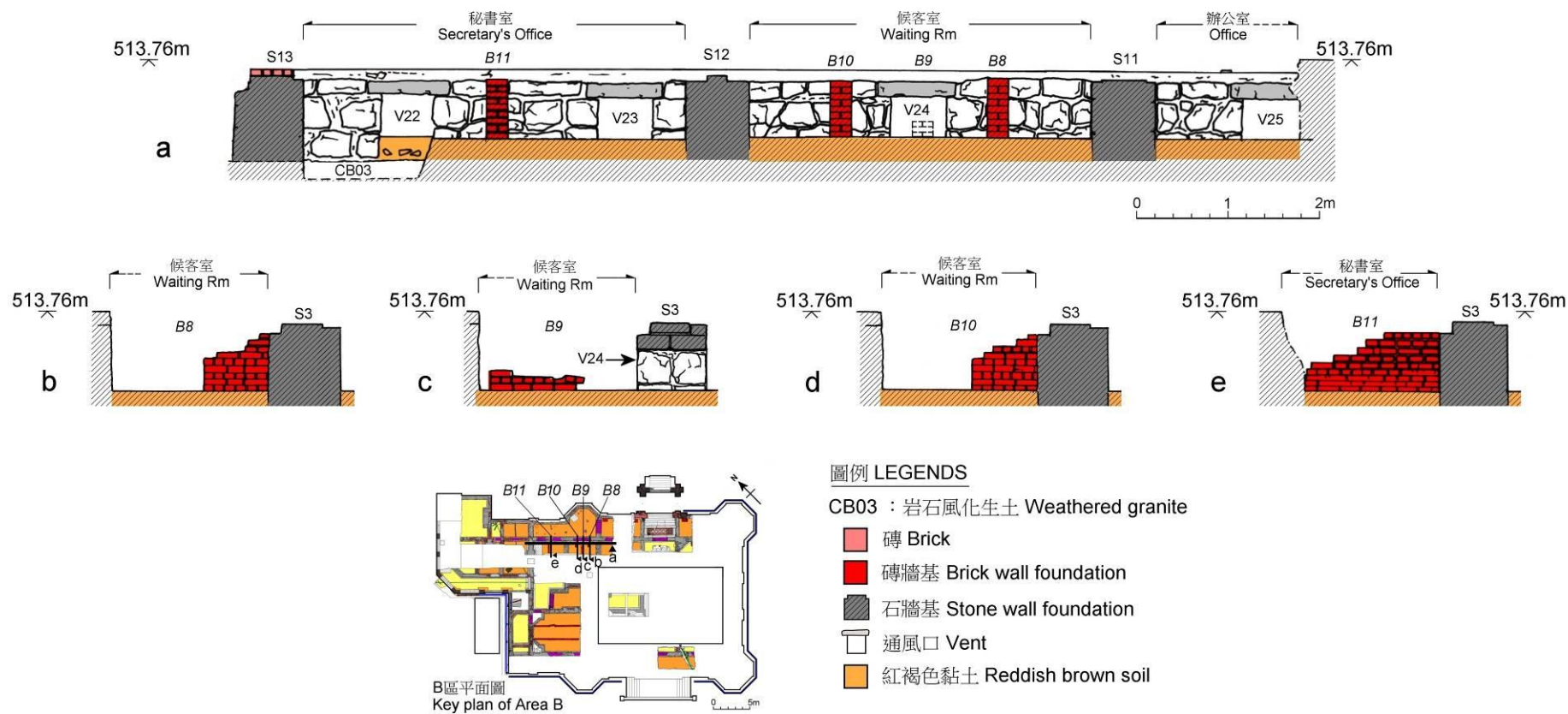
圖 54 磚牆基 B8, B9, B10 及 B11 側視圖 Fig 54 Side views of brick wall foundations B8, B9, B10 and B11
