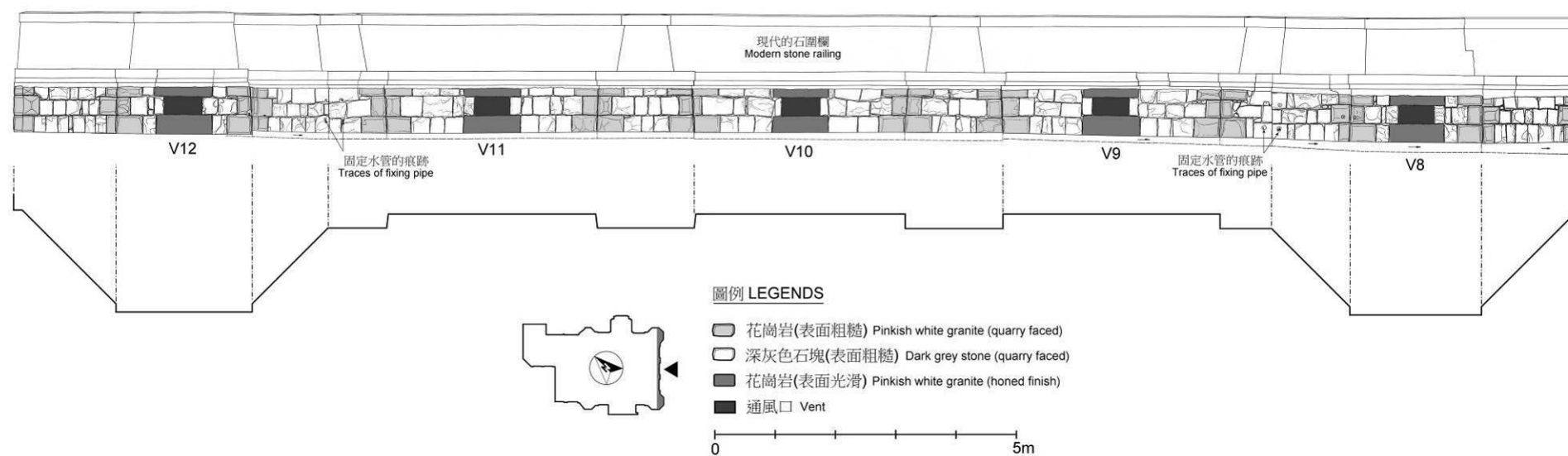
圖 29 前總督山頂別墅東面的外石牆基 Fig 29 Eastern stone wall foundation of Former Mountain Lodge
