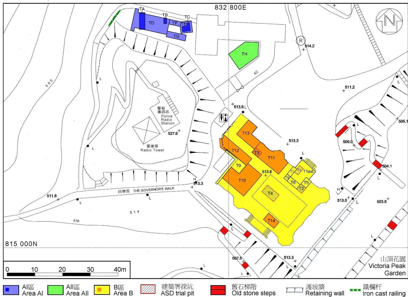
圖 1 2008 年前總督山頂別墅考古調查平面圖 Fig 1 Archaeological investigation plan of Former Mountain Lodge, 2008
