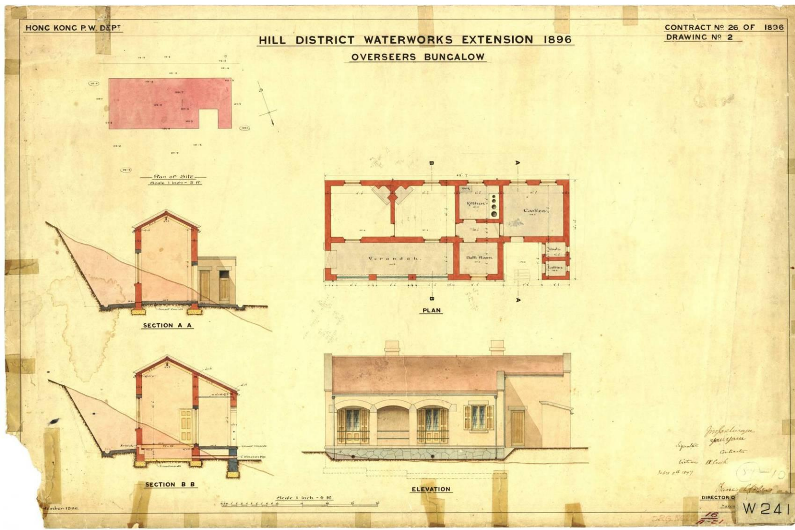
17. 1896 年舊水務署平房平面圖 Plan of the Hill District Waterworks Extension, Overseer Bungalow, 1896
