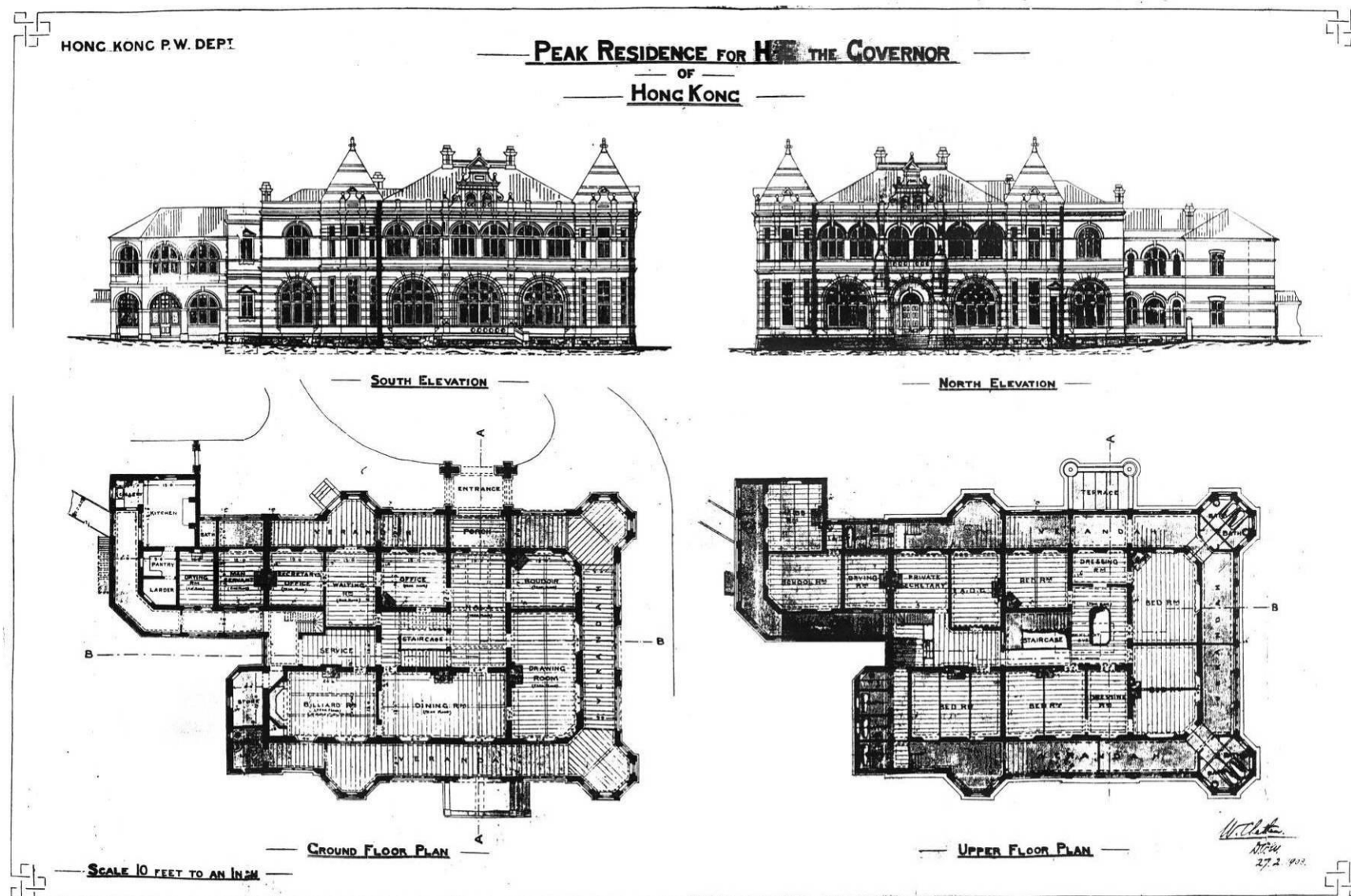
1. 1903 年前總督山頂別墅的平面圖 Plan of Former Mountain Lodge, 1903
