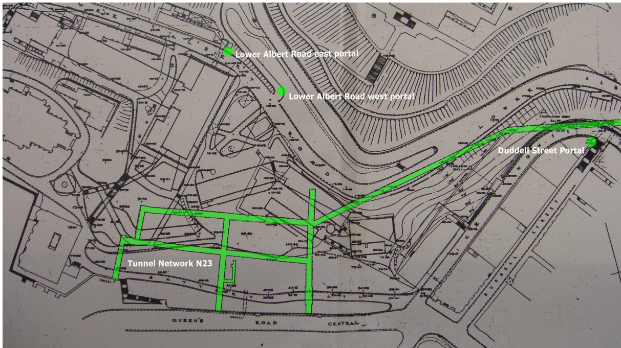
A plan highlighting the tunnels under the CGO and the tunnel portals
